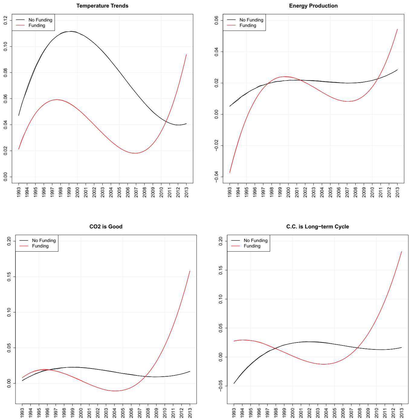
Fig. 4. The influence of corporate funding on themes within the climate change contrarian movement, 1993–2013. The y axis indicates how much a topic was written about. The red line represents the prevalence of the topic in the texts of contrarian organizations who received money, and the black line represents the prevalence of the topic for contrarian organizations who did not receive money. Interaction plots of all other topics are provided in SI Appendix .
